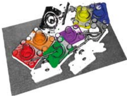
3DMaMA locates seven parts located in 1 second in an occluded scene
