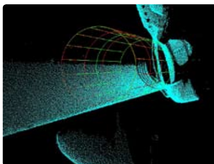
Advanced cylinder fit in a point cloud from the Scorpion 3D Modeller.
