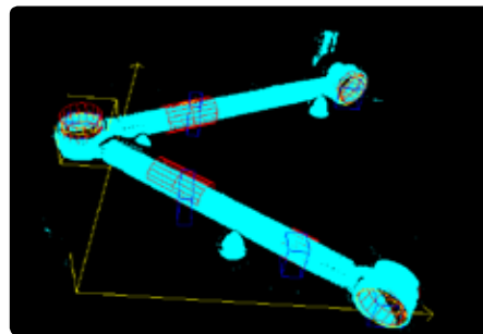
Measurement on an automotive V-stay with the Scorpion 3D Modeller
