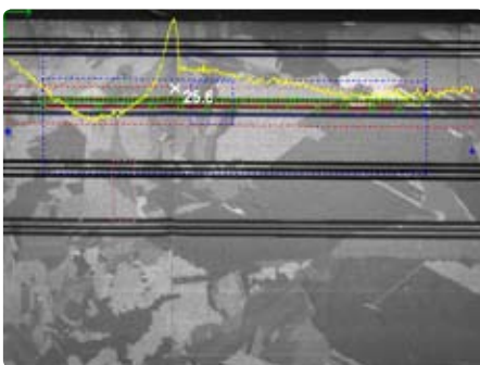
Screen image showing typical sawmark changes across a solar cell wafer. A 25.6 µm sawmark is found.
